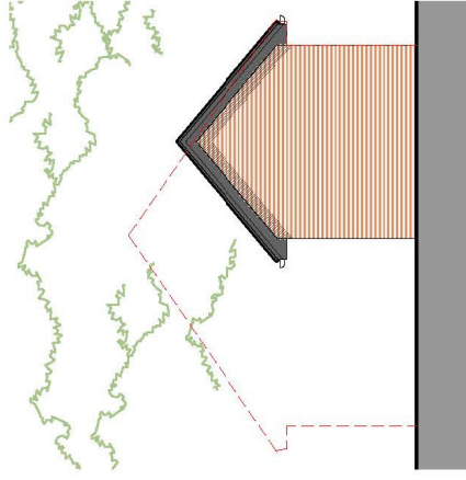
Rear elevation 1:100
